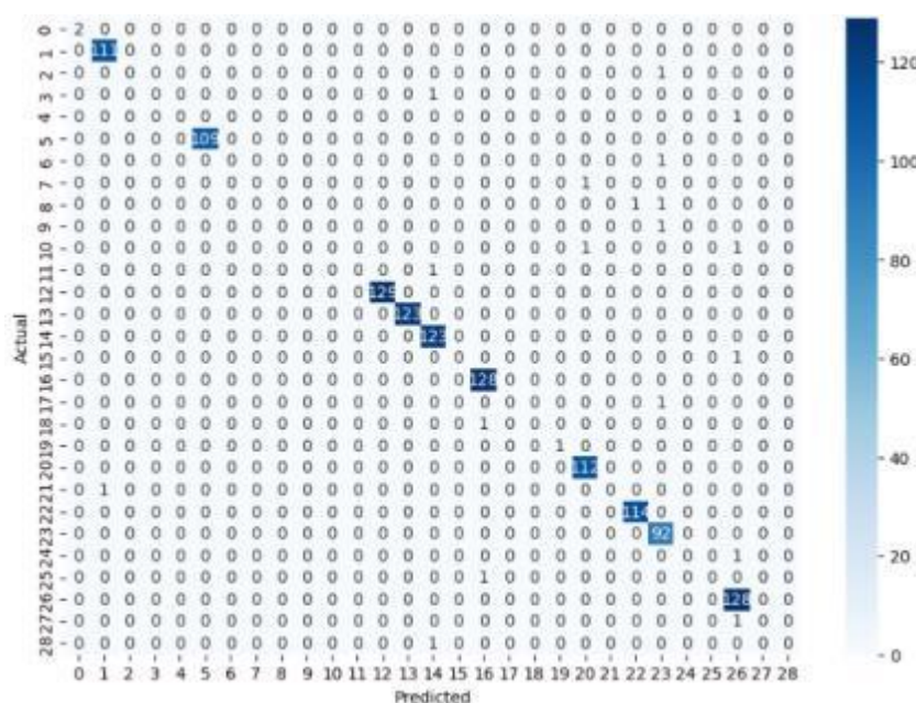
Figure 2. Confusion Matrix
