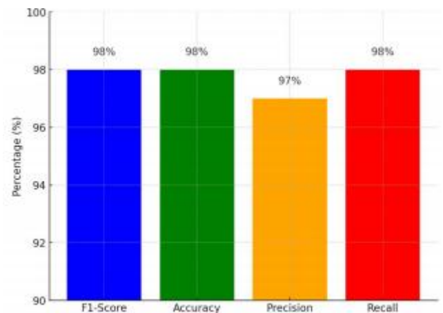
Figure 1. Model Performance.
